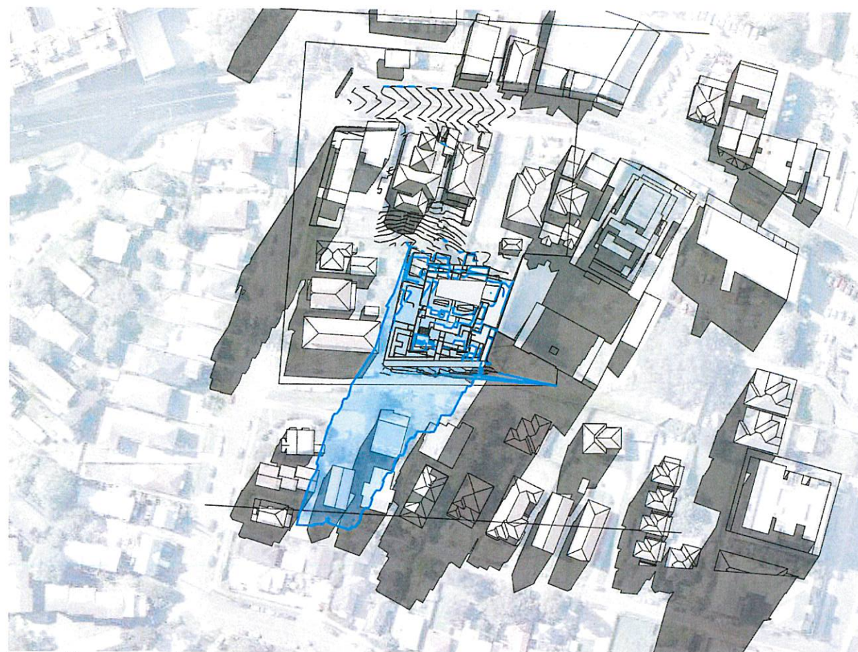
Shadow 10 am - proposed SCALE 1:2000
