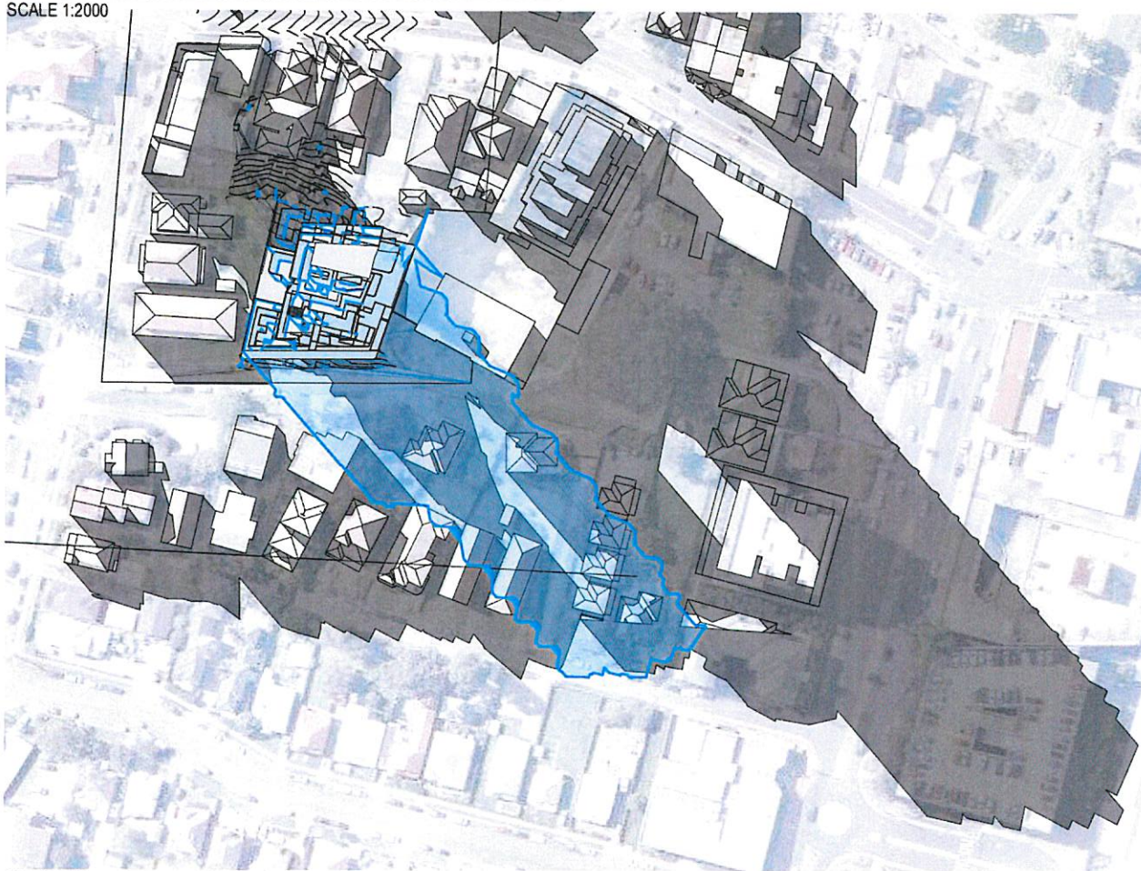
Shadow 3pm - proposed
